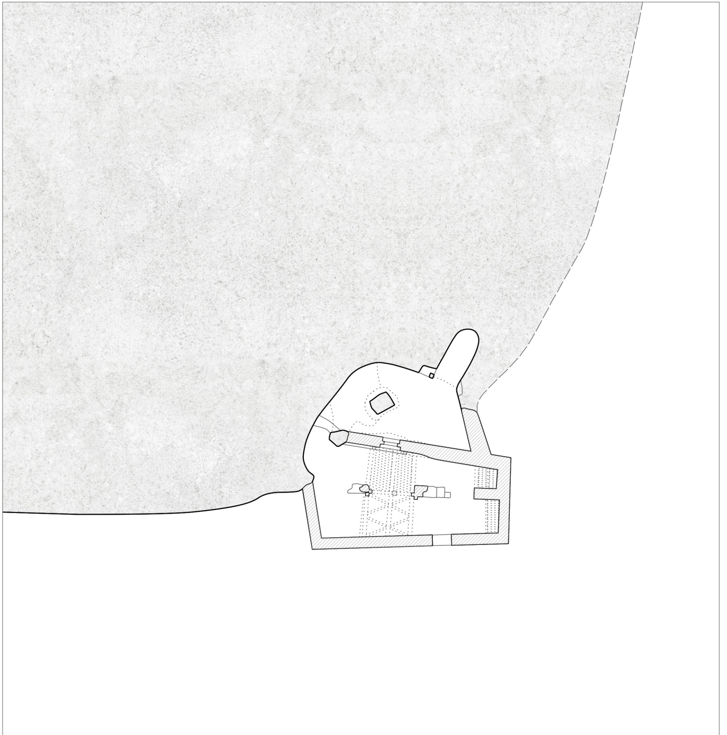
Agwaza Old Church Ground Floor Plan (2017)
